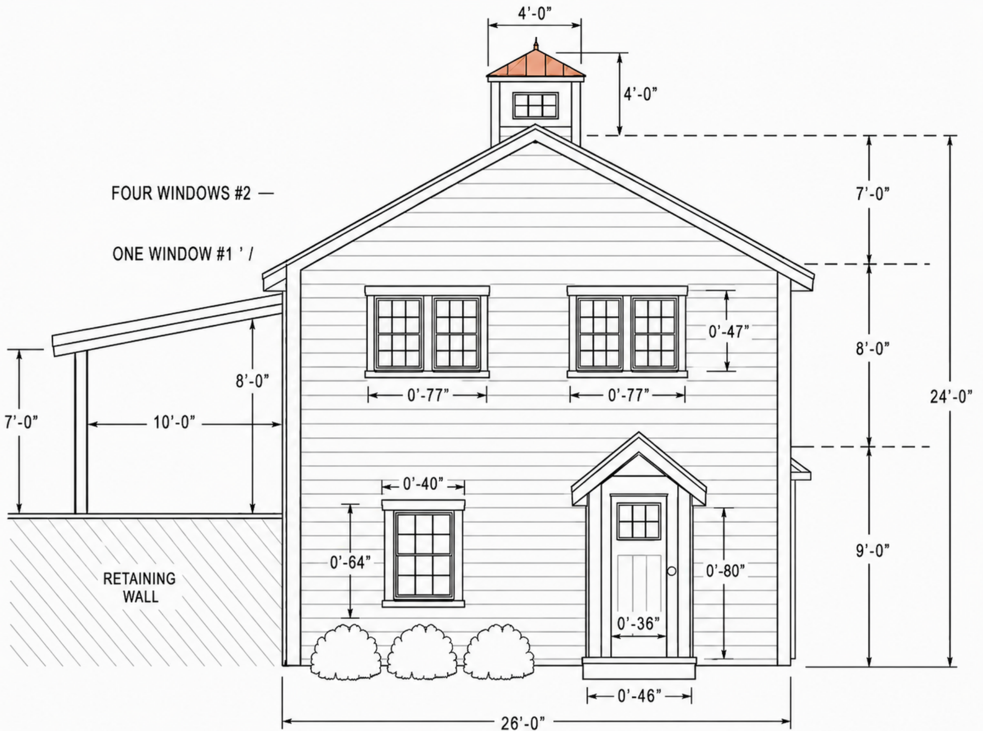
FRONT ELEVATION
